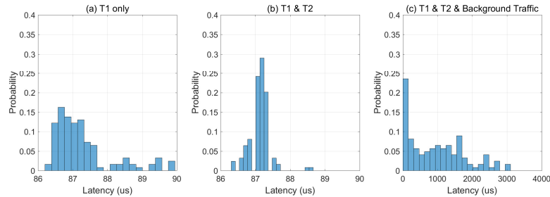
Fig. 8. The probability distribution of latency of T1 when: (a) serving only T1; (b) serving T1 and T2; (c) serving T1 and T2 with background traffic on both channels.
